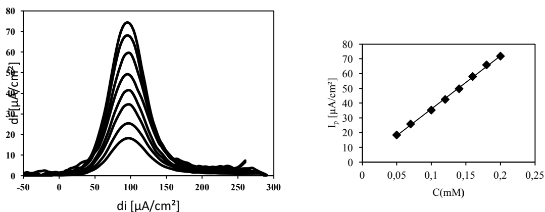
Fig. 6: Calibration curves of Dopamine on the surface of the L-His sonogel-carbon electrode. Phosphate buffer 0.05\text{M} at \text{pH} = 7.4 .
