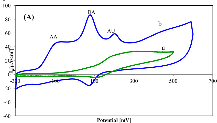
Fig. 11: Cyclic voltammograms for mixture of 8 \times 10^{-7} \text{M} UA, 4 \times 10^{-4} \text{M} AA and 4 \times 10^{-6} \text{M} DA in 0.05M phosphate buffer pH7.4 at (a) unmodified electrode, (b) L-Histidine sonogel-carbone modified electrode. Scan rate of 100 \text{mVs}^{-1} and T=25^\circ\text{C}
