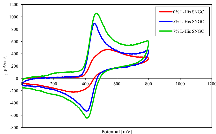
Fig.4: Cyclic voltammograms of 10^{-3} M DA in 0.05M phosphate buffer pH 2 at unmodified sonogel-carbon electrode, 5% L-His sonogel-carbon modified electrode and 7% L-His sonogel-carbon modified electrode. The scan rate is 100mV/s.
