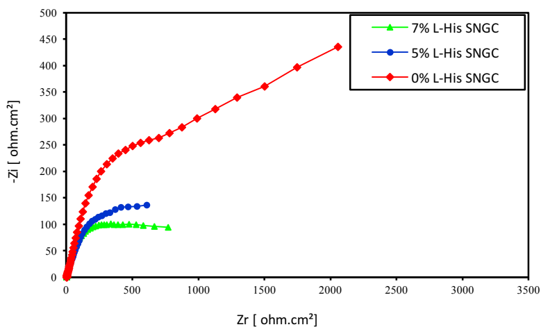
Fig.3: Nyquist diagram of 10 -3 M DA 0.05M phosphate buffer of pH=2 using different electrodes at the oxidation of DA unmodified sonogel-carbon electrode, 5% L-His sonogel-carbon modified electrode and 7% L-His sonogel-carbon
