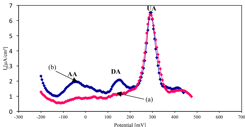
Fig.13. SWV at 7%L-His modified electrode (a): serum diluted 60 fold. (b): serum diluted 60 fold contained 8 \times 10^{-6} M DA and 2 \times 10^{-4} M AA.
