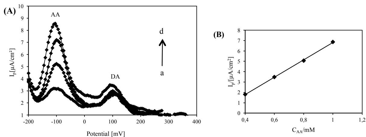
Fig. 9: (A) SWV at 7%L-histidine sonogel carbon modified electrode in pH 7.4 PBS containing 410^{-6} M DA in the presence of different concentrations of AA(a-d) : 4 \times 10^{-4} , 6 \times 10^{-4} , 8 \times 10^{-4} and 1 \times 10^{-3} M. Scan rate: 100 \text{mVs}^{-1}
