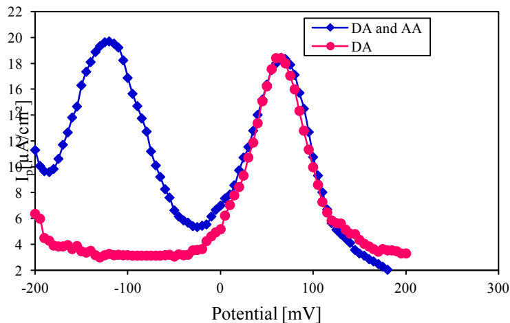
Fig. 8: SWVs for 5 \times 10^{-5}\text{M} DA and 2 \times 10^{-3}\text{M} AA at 7% L-His sonogel-carbon modified electrode in 0.05M pH 7.4 PBS.
