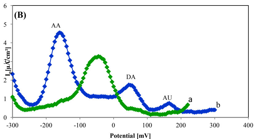
Fig.12: SWV of 4 \times 10^{-6} \text{M} DA, 4 \times 10^{-4} \text{AA} and 8 \times 10^{-7} \text{M} UA mixtures at (a) unmodified electrode, (b) L-Histidine sonogel-carbon modified electrode in 0.05M phosphate buffer (pH 7.4). Pulse amplitude: 25mV
