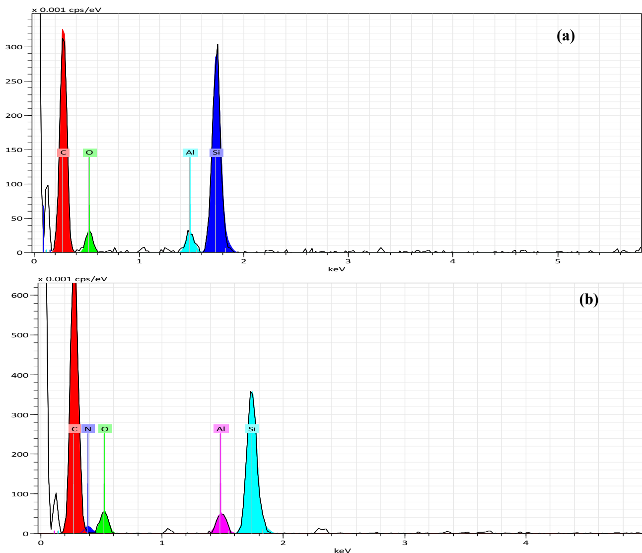
Fig. 2: (a) EDS spectrum of a unmodified Sonogel-Carbon electrode; (b) EDS spectrum of a 7% L-His Sonogel-Carbon modified electrode.
