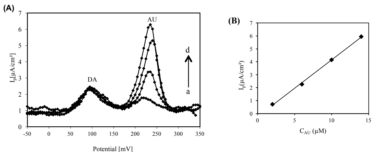
Fig.10: SWV voltammograms corresponding to the interference studies when dopamine (DA) is determined in the presence of uric acid (UA) at L-His sonogel carbon modified electrode. Concentration of DA is constant ( 410^{-6} M), and concentration of UA is varied (a-d): 2 \times 10^{-6} , 6 \times 10^{-6} , 10^{-5} and 1.4 \times 10^{-5} M. Scan rate: 100 \text{mVs}^{-1} . pH7.4
