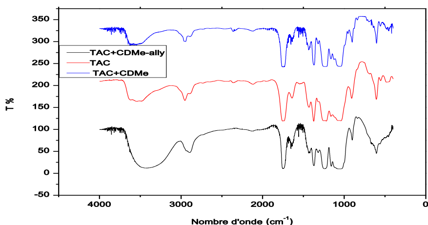
Figure 2: FT-IR spectrum of membranes.
