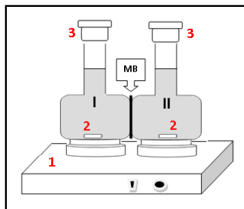
Figure 1: Schematic representation of the dialysis cell.
