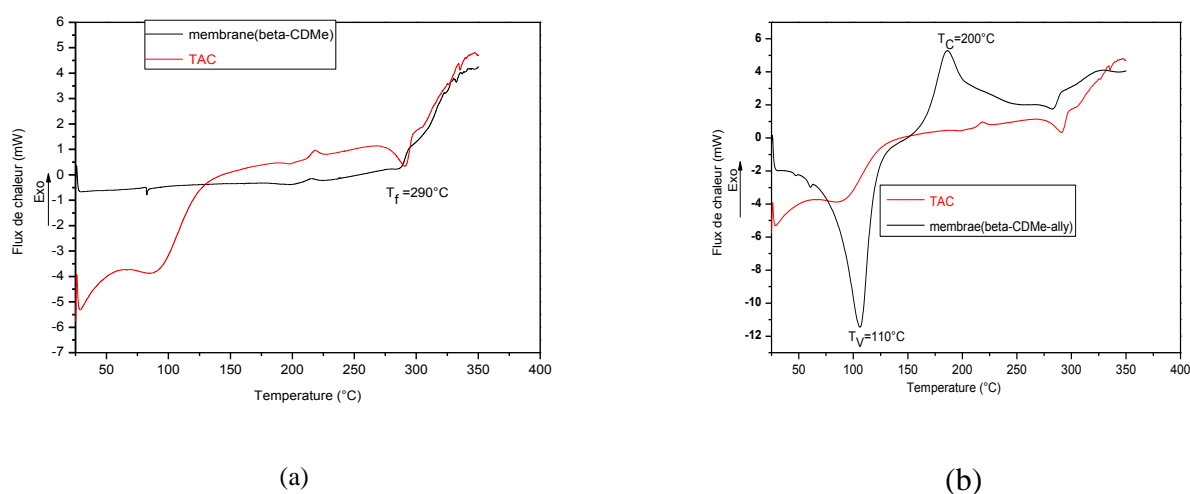
Figure 4: \beta -CDMe (a) and \beta -CDMe-ally membranes (b)
