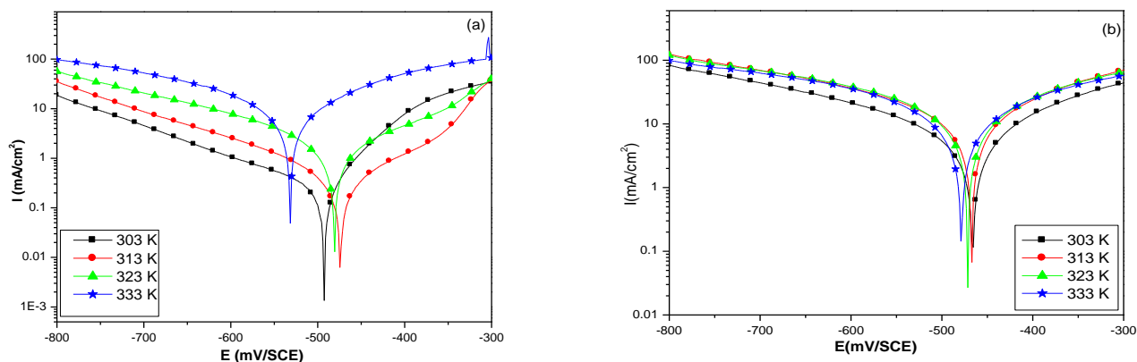
Figure 5: Polarization curves of carbon steel in 2M H_3PO_4 with (a) and without (b) 10^{-3} M of MTTT for various temperatures
