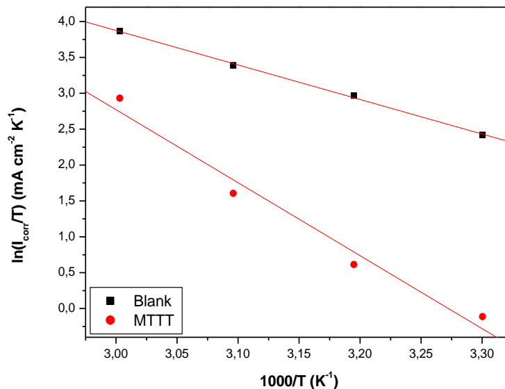
Figure 7: Transition-state plots for carbon steel current density ( I_{\text{corr}} ) in 2M \text{H}_3\text{PO}_4 in absence and in presence of 10^{-3}\text{M} of MTTT.
