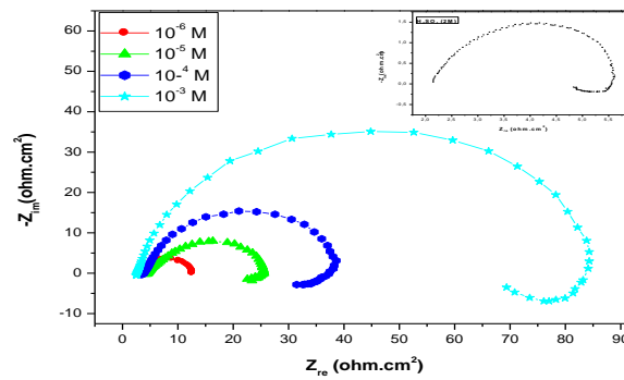
Figure 3: Nyquist diagrams for carbon steel in 2M H 3 PO 4 containing different concentrations of MTTT at 303K.
