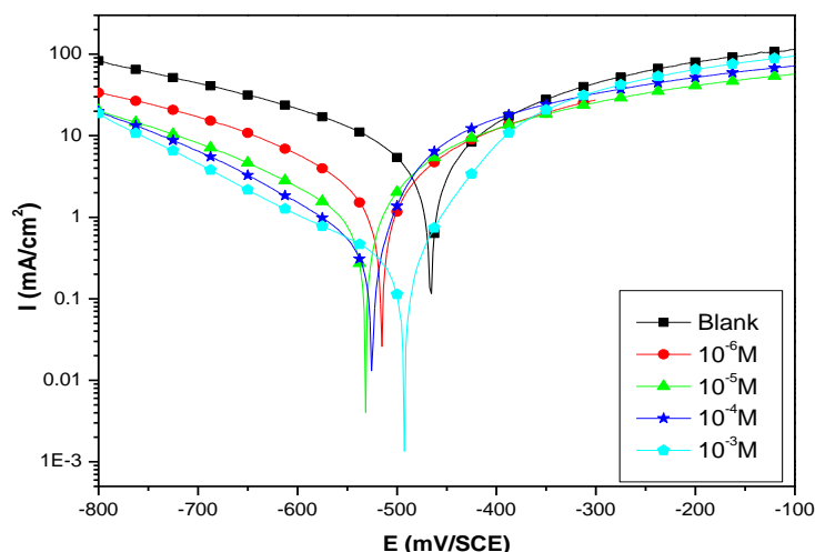
Figure 2: Potentiodynamic polarization curves of carbon steel in 2M H 3 PO 4 in the presence of different concentrations of MTTT at 303K.
