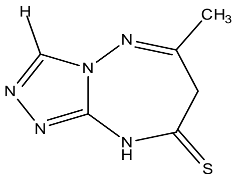
Figure 1: The molecular structure of 6-methyl-7H-1,2,4-triazolo[4,3b][1,2,4]-triazepine-8(9H)-thione (MTTT).
