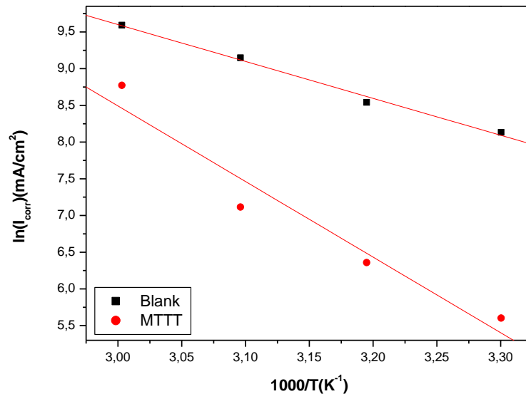
Figure 6: Arrhenius plots for carbon steel corrosion current density ( I_{\text{corr}} ) in 2M \text{H}_3\text{PO}_4 in absence and in presence of 10^{-3}\text{M} of MTTT.
