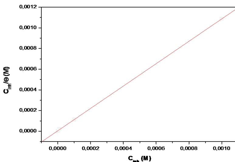
Figure 8: Langmuir isotherm adsorption model of MTTT on the carbon steel surface in 2M \text{H}_3\text{PO}_4 .
