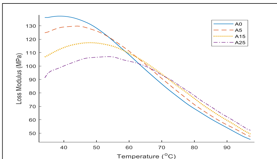
Figure 2: Variation of loss modulus with temperature of PPP-RPP composites at 1 Hz.
