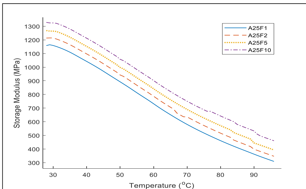
Figure 4: Variation of storage modulus with temperature of PPP-RPP composites at different frequencies.
