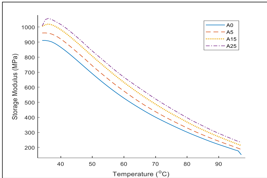
Figure 1: Variation of storage modulus with temperature of PPP-RPP composites at 1 Hz
