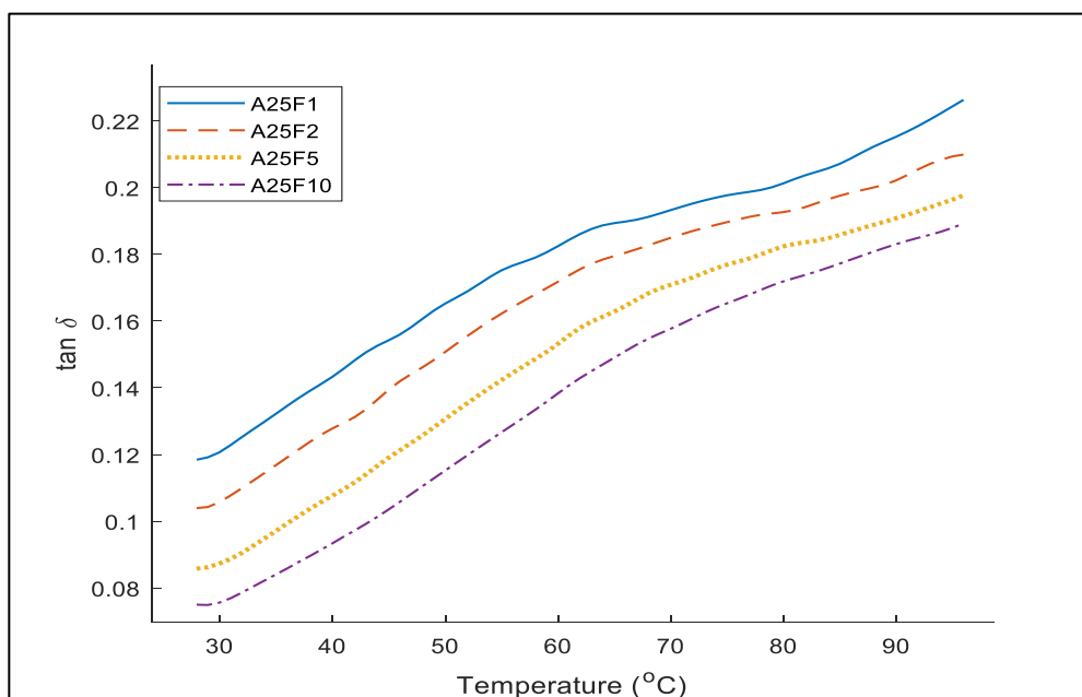
Figure 6: Variation of loss modulus with temperature of PPP-RPP composites at different frequencies.
