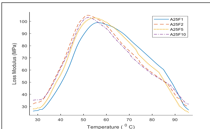
Figure 5: Variation of loss modulus with temperature of PPP-RPP composites at different frequencies.
