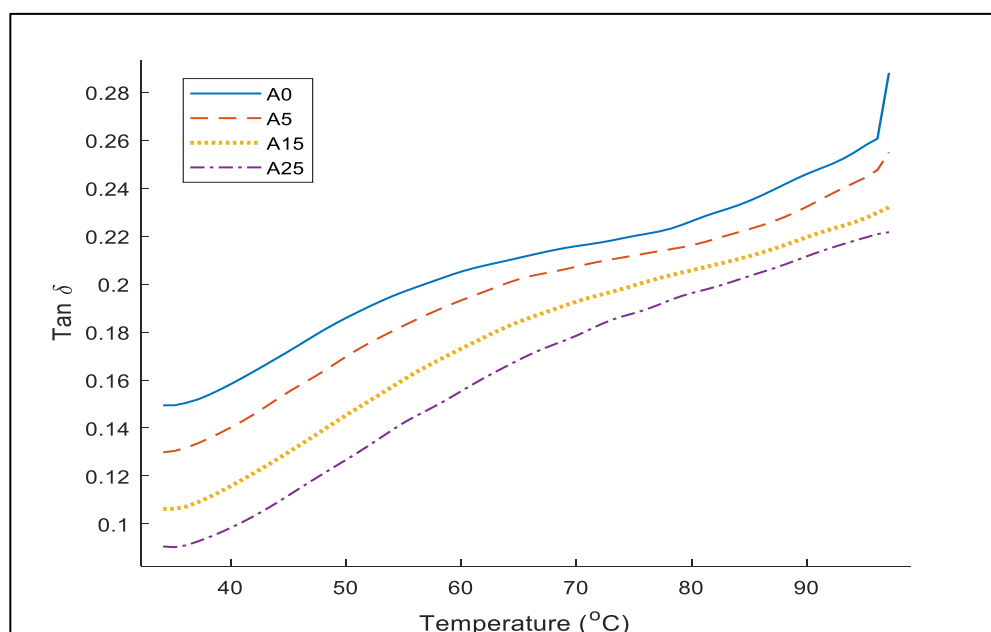
Figure 3: Variation of damping parameter with temperature of PPP-RPP composites at 1 Hz.
