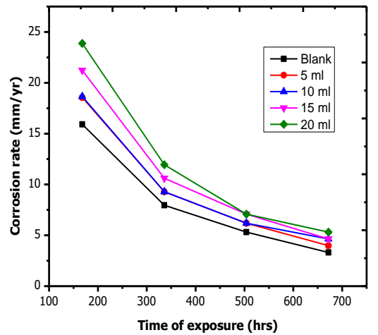
Figure 8. Corrosion rate of mild steel against exposure time for Moringa oleifera seed extract in 1.0 M NaOH.
