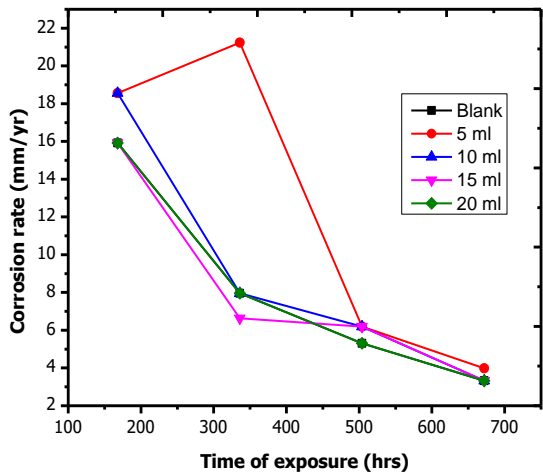
Figure 7. Corrosion rate of mild steel against exposure time for Moringa oleifera leaf extract in 1.0 M NaOH.
