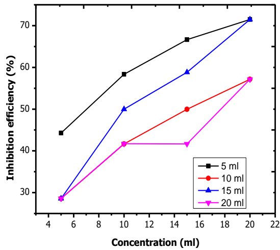
Figure 11. Inhibition efficiency against concentration of Moringa oleifera leaf extract on the mild steel in 1.0 M H 2 SO 4 .
