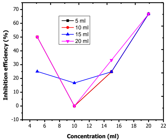
Figure 13. Inhibition efficiency against concentration of Moringa oleifera leaf extract on the mild steel in 0.5 M NaOH.
