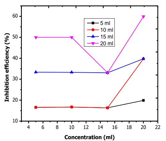
Figure 16. Inhibition efficiency against concentration of Moringa oleifera seed extract on the mild steel in 1.0 M NaOH.
