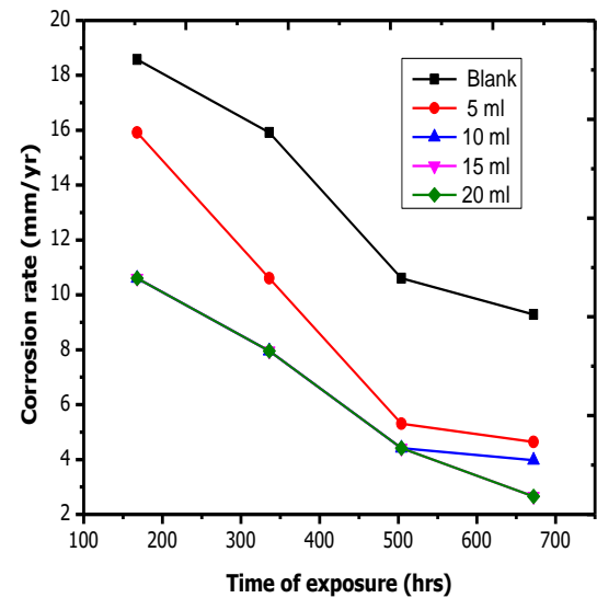
Figure 4. Corrosion rate of mild steel against exposure time for Moringa oleifera seed extract in 1.0 M H 2 SO 4 .
