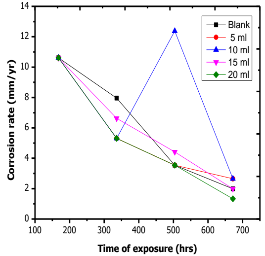
Figure 6. Corrosion rate of mild steel against exposure time for Moringa oleifera seed extract in 0.5 M NaOH.
