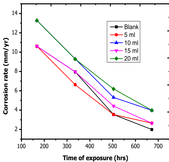
Figure 3. Corrosion rate of mild steel against exposure time for Moringa oleifera leaf extract in 1.0 M H 2 SO 4 .
