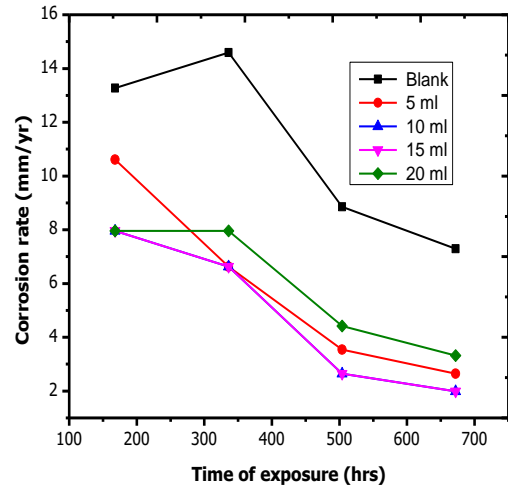
Figure 2. Corrosion rate of mild steel against exposure time for Moringa oleifera seed extract in 0.5M H 2 SO 4 .
