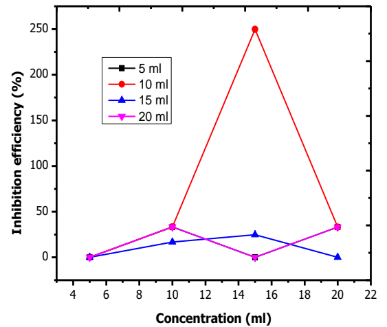
Figure 14. Inhibition efficiency against concentration of Moringa oleifera seed extract on the mild steel in 0.5 M NaOH.
