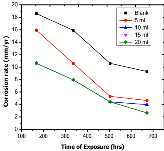
Figure 1. Corrosion rate of mild steel against exposure time for Moringa oleifera leaf extract in 0.5M H 2 SO 4 .
