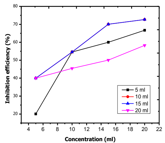
Figure 10. Inhibition efficiency against concentration of Moringa oleifera seed extract on the mild steel in 0.5 M H 2 SO 4
