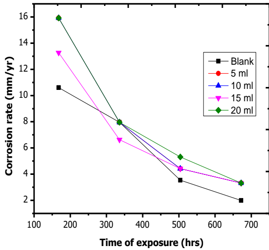
Figure 5. Corrosion rate of mild steel against exposure time for Moringa oleifera leaf extract in 0.5 M NaOH.
