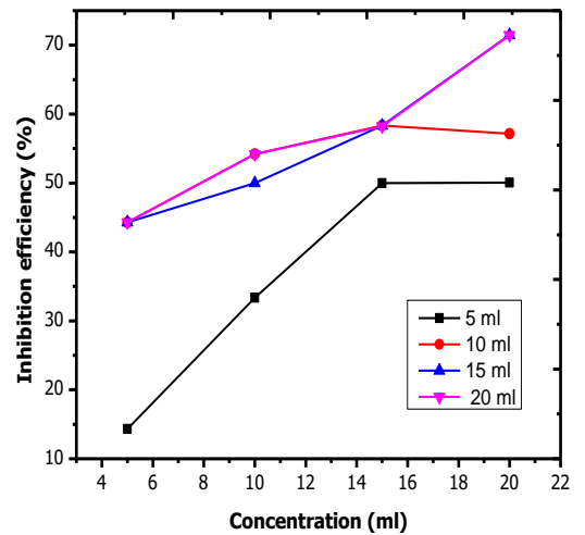
Figure 12. Inhibition efficiency against concentration of Moringa oleifera seed extract on the mild steel in 1.0 M H 2 SO 4 .
