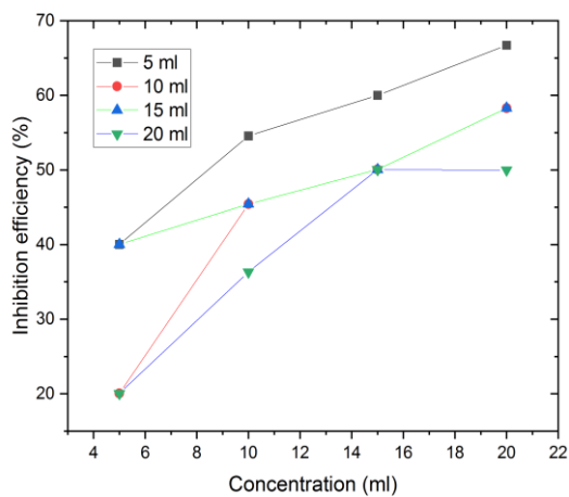
Figure 15. Inhibition efficiency against concentration of Moringa oleifera leaf extract on the mild steel in 1.0 M NaOH.
